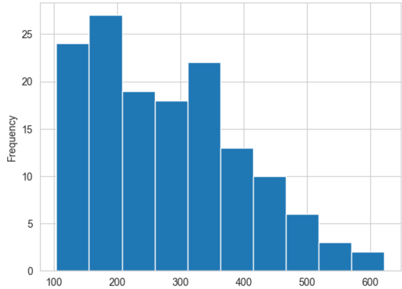
TS Histogram
