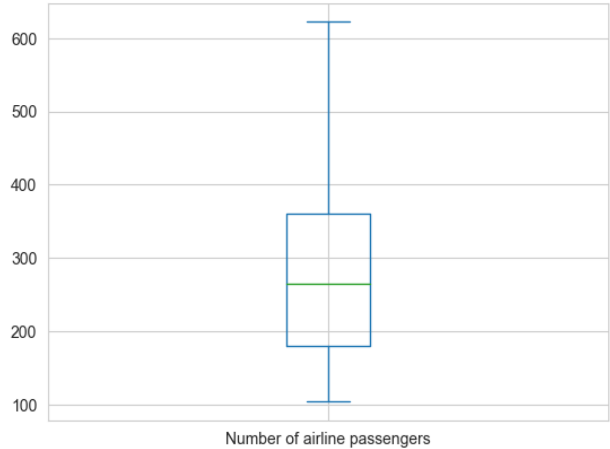
TS BoxPlot
