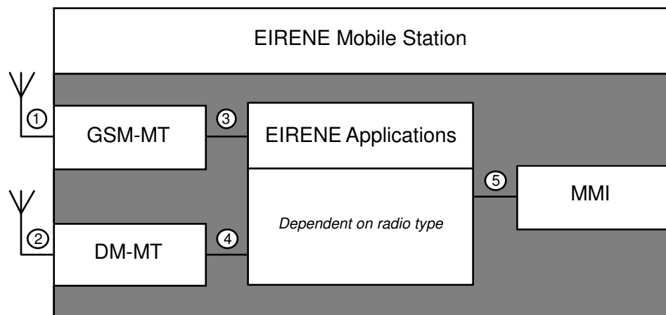
Figure 4-1: Logical mobile radio architecture and interfaces
