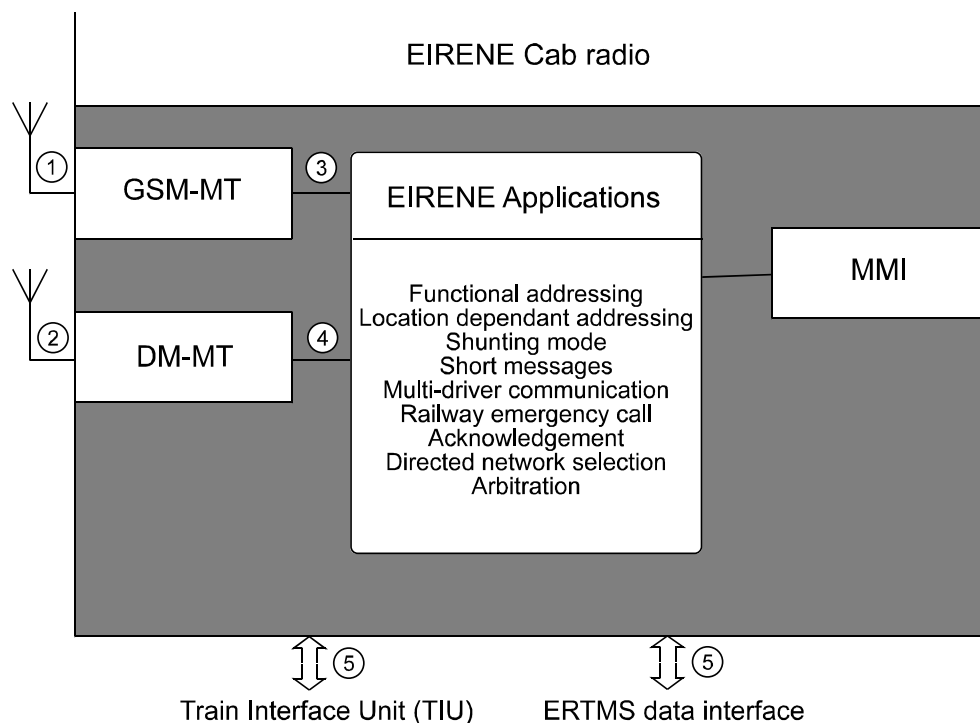
Figure 5-1: Logical Cab radio architecture and interfaces
