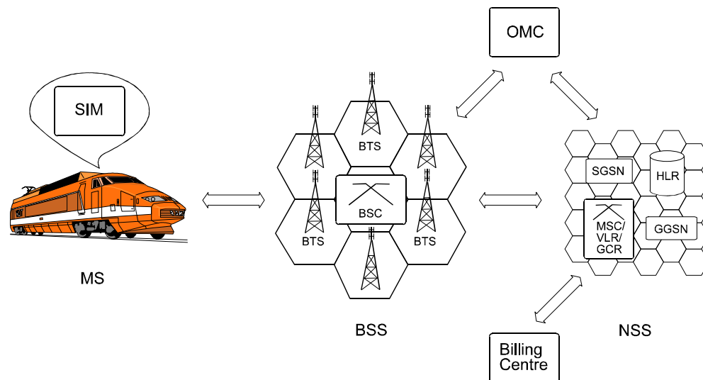
Figure 1-3: GSM architecture overview
