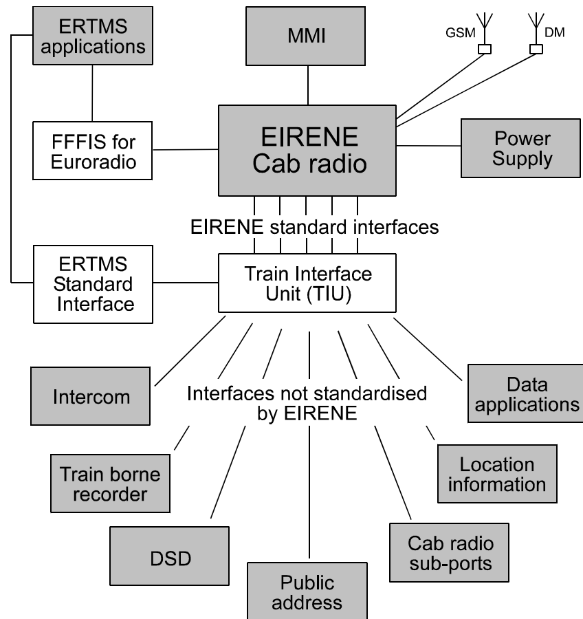
Figure 5-3: Interfaces to the Cab radio
