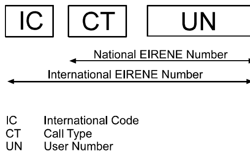
Figure 9-2: International EIRENE Number structure
