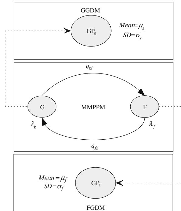
Fig. 2. Transaction simulator.
