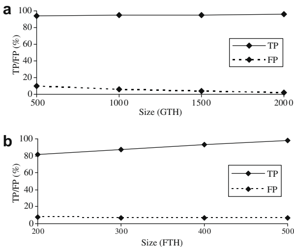
Fig. 4. Variation of TP/FP with (a) size of GTH; (b) size of FTH.
