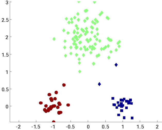
Optimal Clustering
