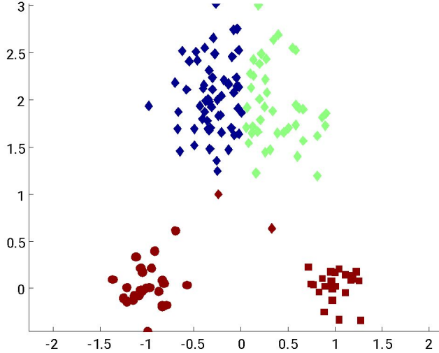
Sub-optimal Clustering
